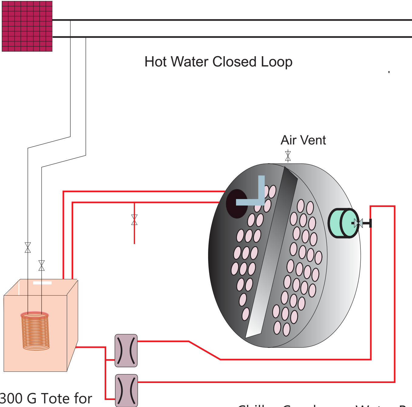
Chiller Condenser Water Box With Temporary Stand Pipe and Blind Flange with Fittings for Chemical Feed Lines
